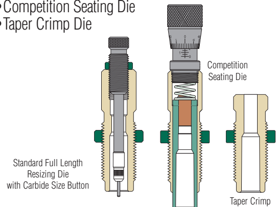
Taper Crimp
